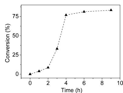
Figure 5. Time-dependent conversion of 4-nitrobenzaldehyde as a function of reaction time over unsupported \text{Au}_{25}(\text{Capt})_{18} . Reaction conditions: 0.2 \mu\text{mol} of \text{Au}_{25}(\text{Capt})_{18} nanocluster catalyst in 2 mL of water, 0.025 mmol of 4-nitrobenzaldehyde, and 0.1 mmol of pyridine under 20 bar of \text{H}_2 at 80 °C for 9 h.
