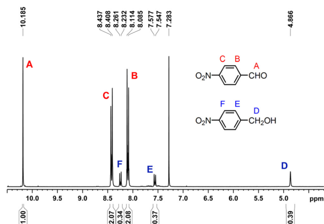
Figure 2. 1 H NMR spectrum of the crude product after the catalytic reaction catalyzed by the \text{Au}_{25}(\text{SG})_{18} nanocluster catalyst. Only residual reactant 4-nitrobenzaldehyde (-CHO at 10.18, the proton on the phenyl ring at 8.44 and 8.41, 8.11, and 8.08 ppm) and the exclusive 4-nitrobenzyl alcohol product (-CH 2 at 4.87, the proton on phenyl ring at 8.26 and 8.23, 7.58, and 7.55 ppm) are found in the spectrum.
