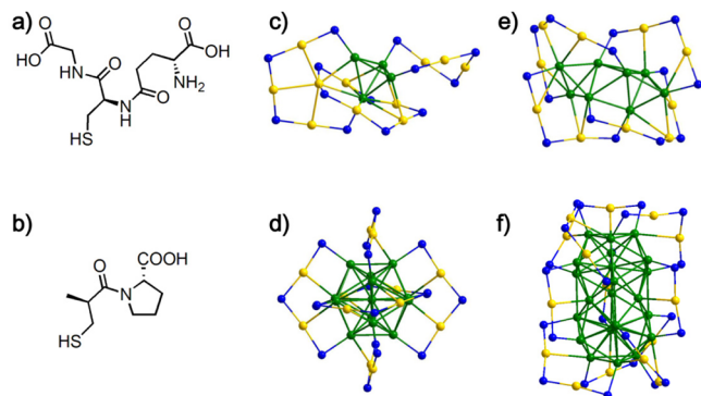
Scheme 1. Molecular Structures of (a) Glutathione and (b) Captopril and Cluster Structures of (c) Au 15 (SR) 13 , 27 (d) Au 25 (SR) 18 , 13 (e) Au 18 (SR) 14 , 28 and (f) Au 38 (SR) 24 14 Nanoclusters a
